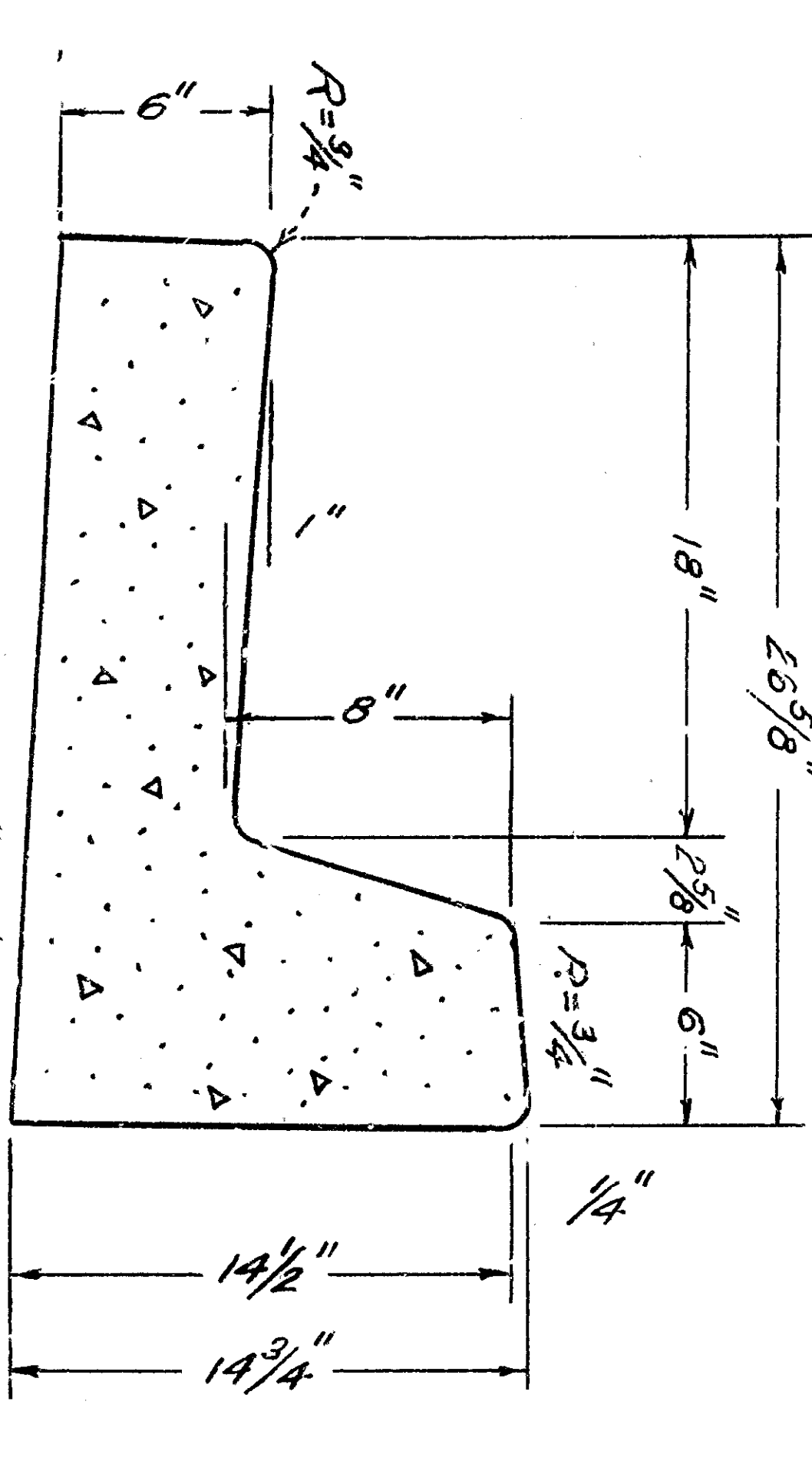
TYPICAL SECTION - PCC CURB & GUTTER
