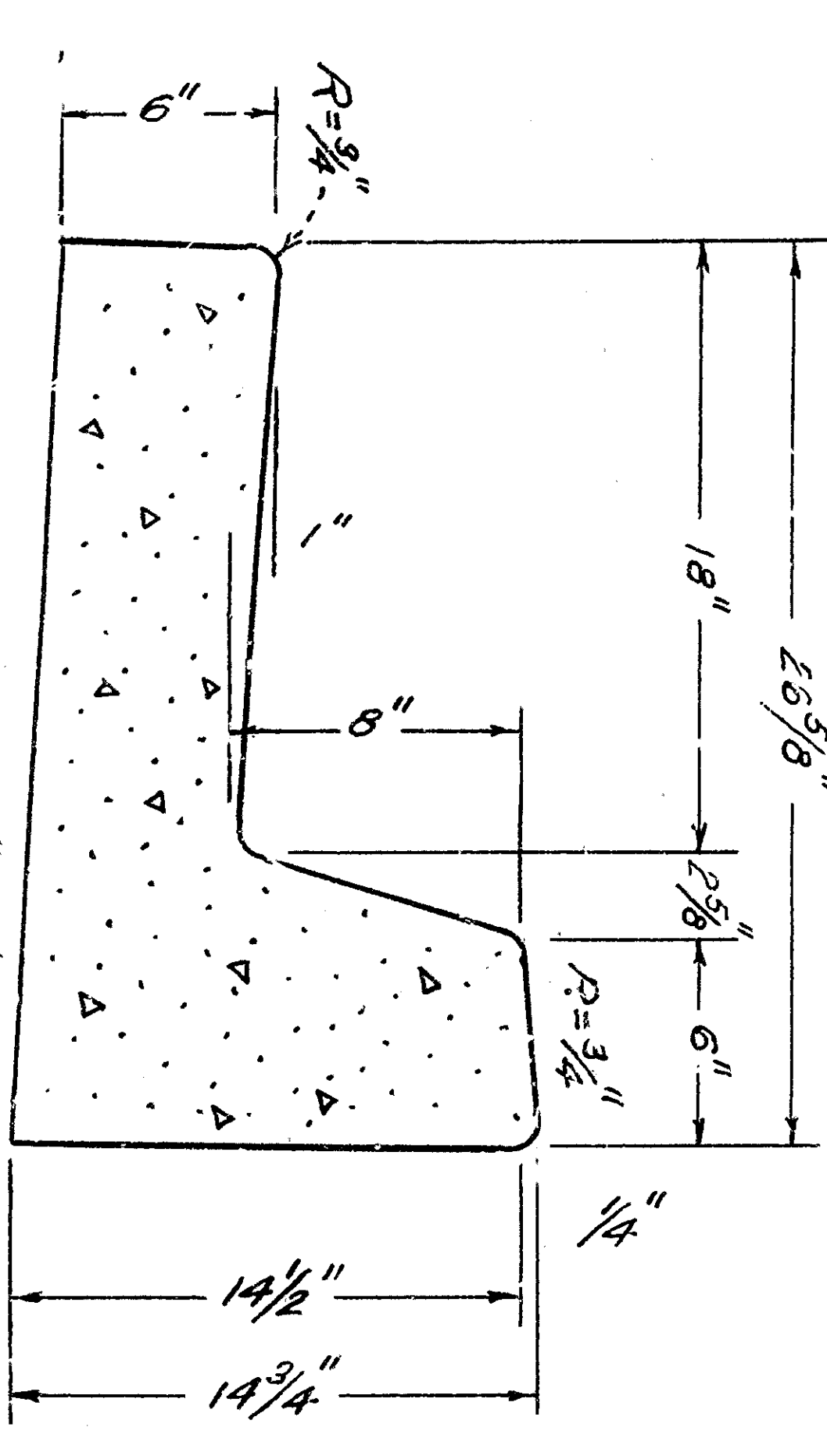
TYPICAL SECTION - PCC CURB & GUTTER
